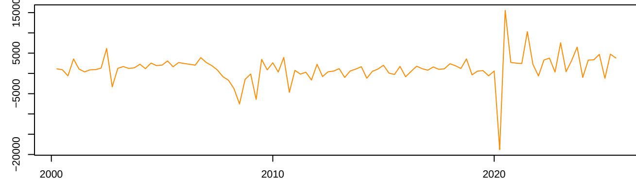
Spain – Stationary
