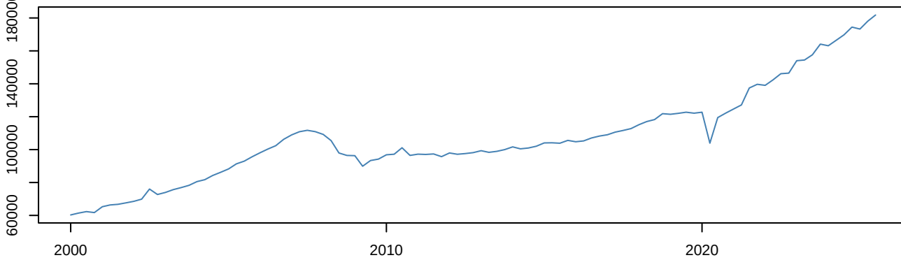
Spain – Raw
