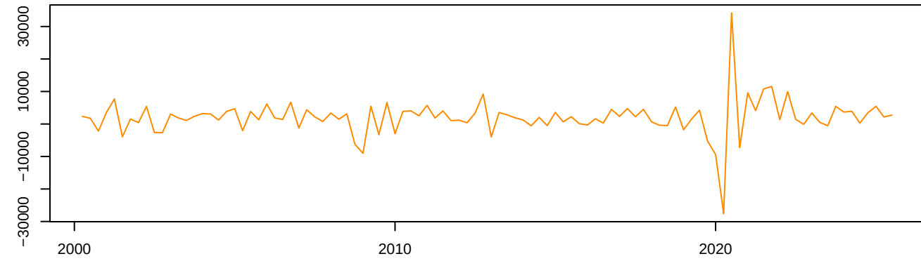
France – Stationary
