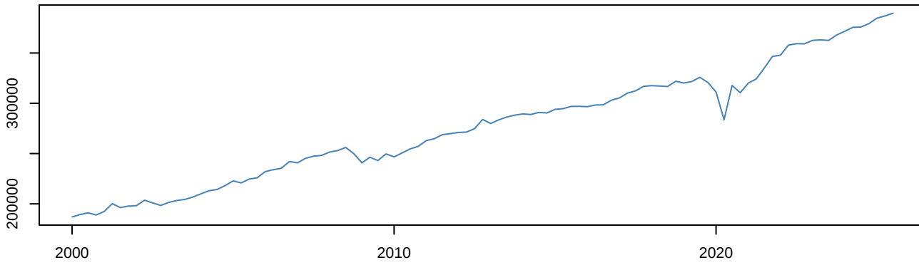
France – Raw
