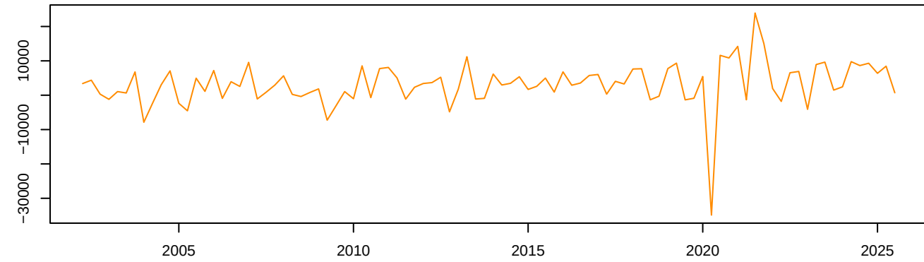
Germany – Stationary
