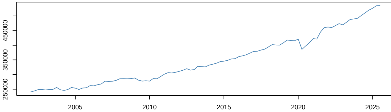
Germany – Raw
