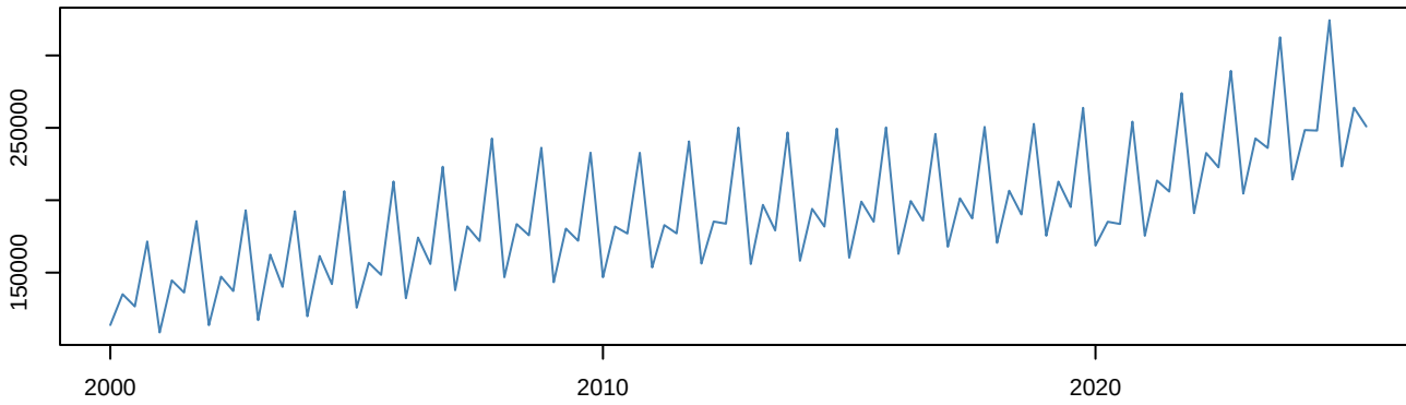
Italy – Raw
