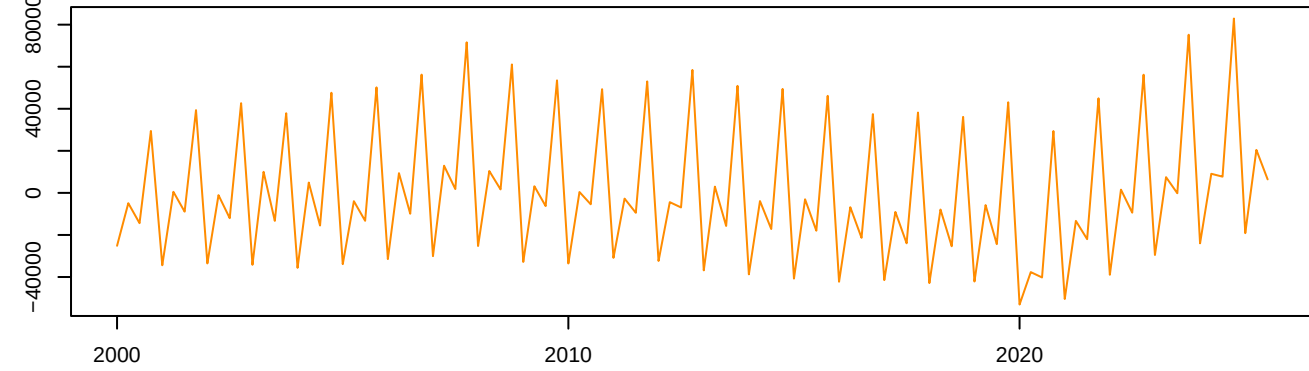
Italy – Stationary
